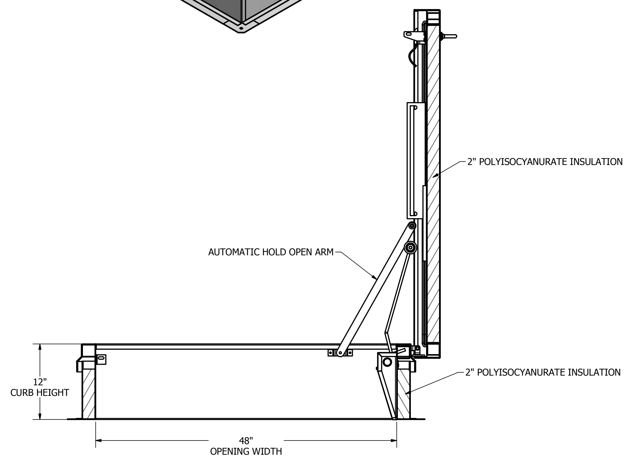
SECTION BT-BT
